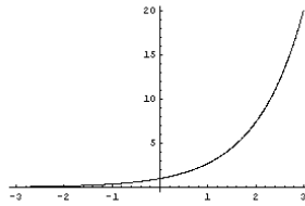
図5 f(x) = \exp(x)
