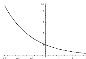
図7 f(x) = \exp(-x/2)
