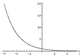
図6 f(x) = \exp(-x)
