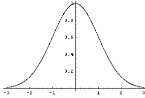
図 8 f(x) = \exp(-x^2/2)
